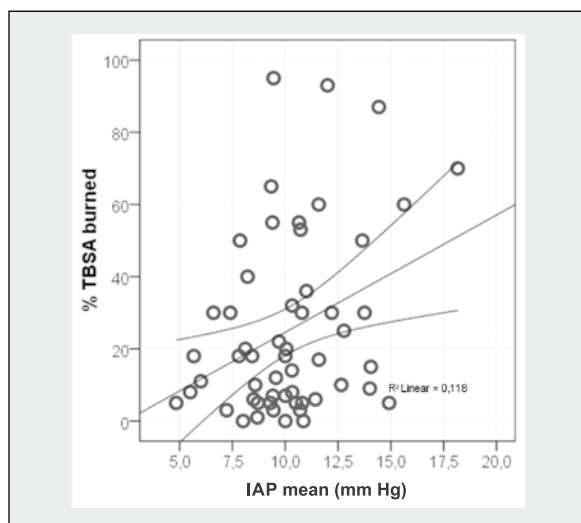
Figure 5. Correlation plot between mean IAP and %TBSA
